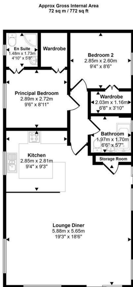
Floorplan
